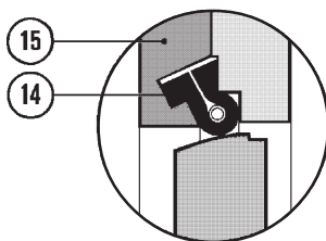
Seal type -85, -86, -88
