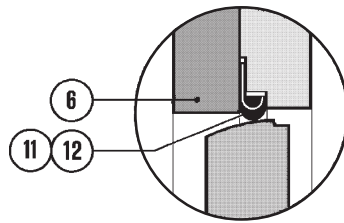
Seal type -55, -66
